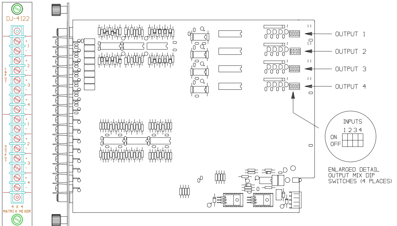
REAR PANEL
